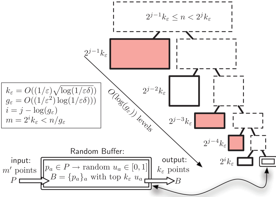
Fig. 1. Illustration of the hybrid summary. The labels at each level of the hierarchy show the number of points represented at that layer. Each filled box contains exactly k_\epsilon summary points, and empty boxes contain no summary points. The random buffer, the bottom left leaf of the hierarchy, is shown in more detail.
